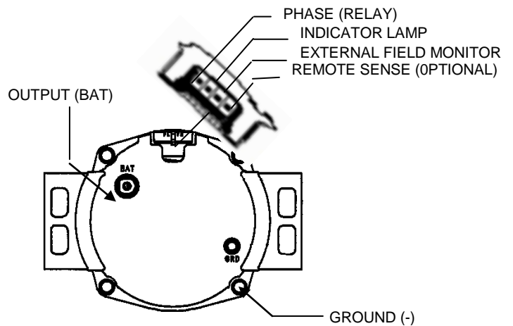
22SI REMOTE SENSE 4-TERMINAL REGULATOR
