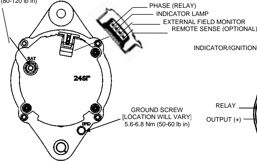
24SI ALTERNATOR
